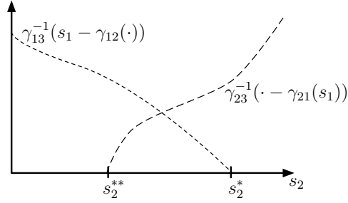
FIG. 9.1. Visualization of (9.2).
