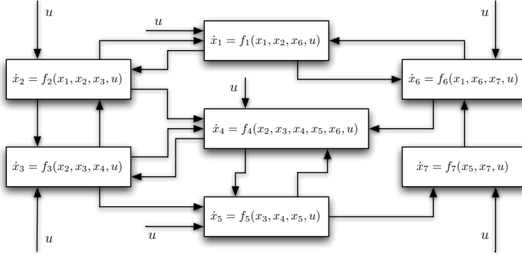
FIG. 2.1. An example of a network of interconnected systems and the associated graph.
