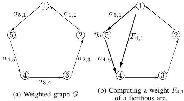
Fig. 3. Cycle network.
