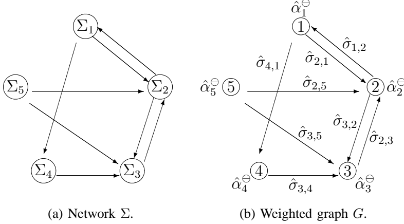
Fig. 1. An example of a general network.
